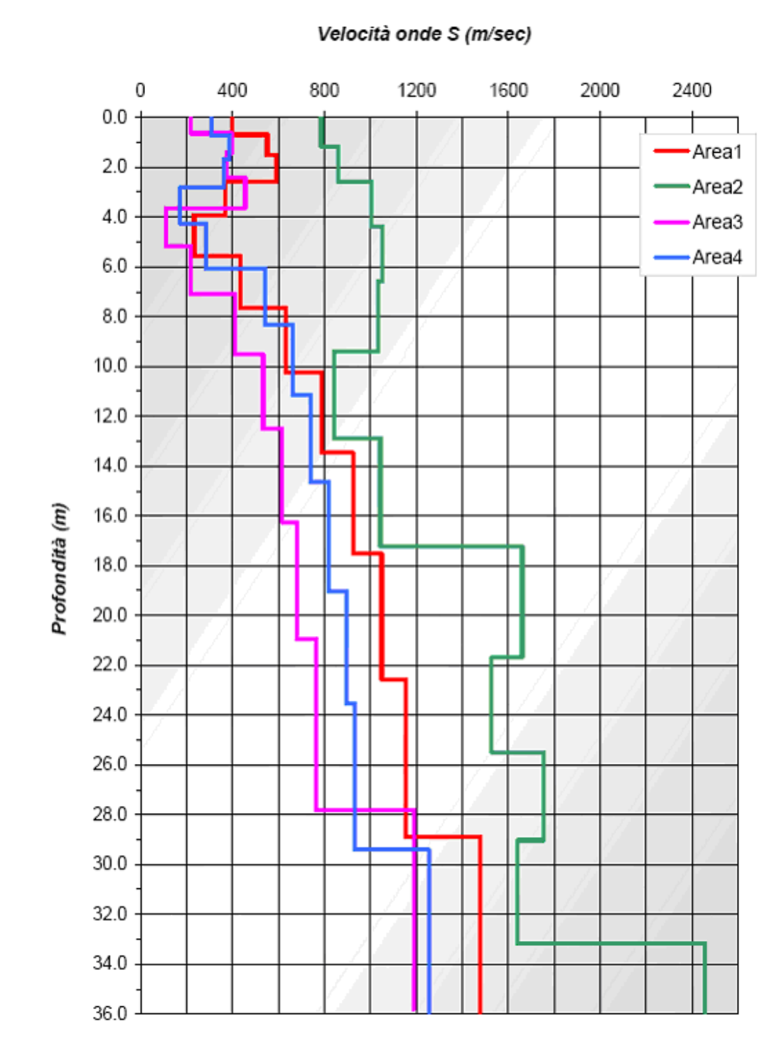
Shear-Wave Velocity Profile from Surface waves inversion
